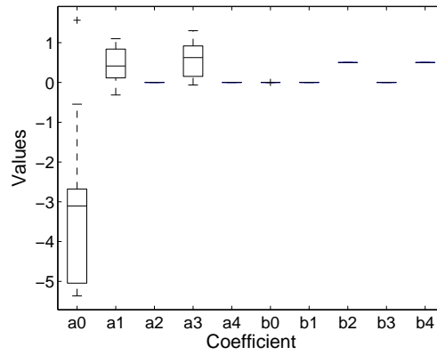
Figure 7.16: Diversity of mean coefficients for pose variation.
