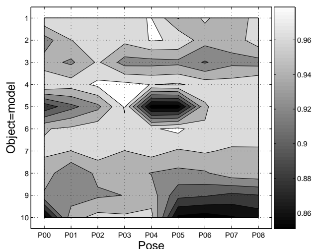
Figure 7.47: CC object=modelexpose array, using LCV.
