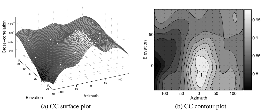
Figure 7.97: CC response under non-linear illumination variation.
