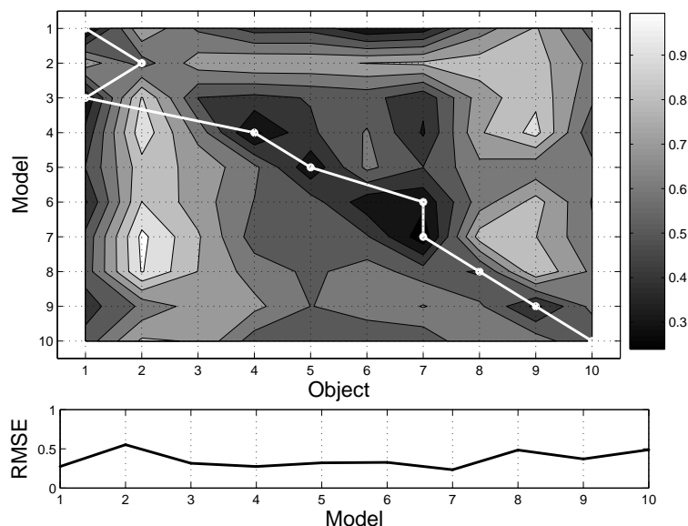
Figure 7.42: RMSE model \times object array for the frontal pose, using AAMs.
