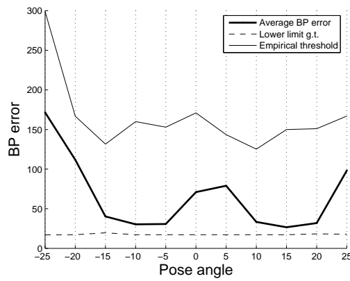
Figure 7.57: Average BP error plot (mode of sample) for moderate noisy case.
