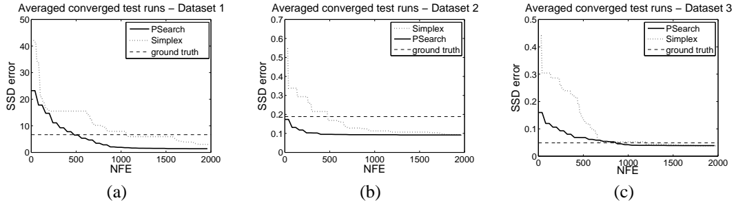
Figure 6.5: The average converged test runs for all the 3 datasets.
