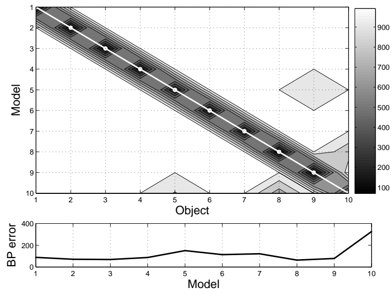
Figure 7.40: BP model \times object array for the frontal pose, using LCV.
