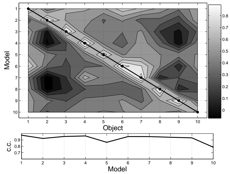
Figure 7.43: CC model \times object array for the frontal pose, using AAMs.
