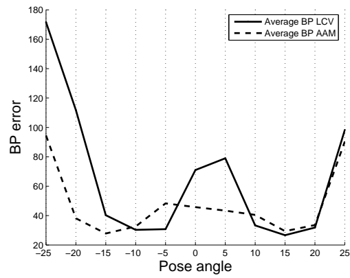
Figure 7.61: Average BP plot (mode of sample) for moderately noisy case.
