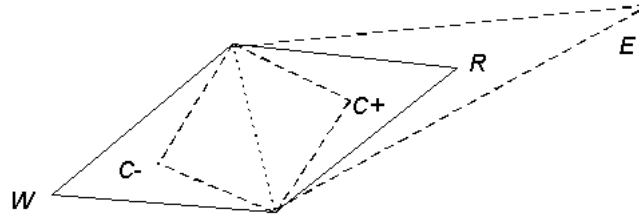
Figure 2.3: Possible simplex moves after the worst point (W) is identified and rejected.
