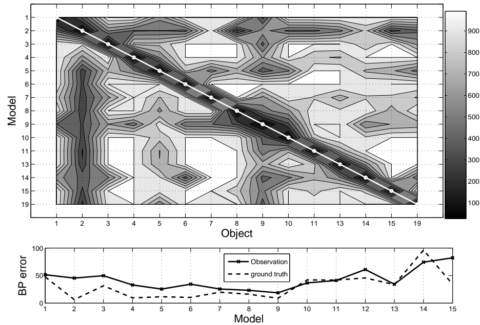
Figure 7.25: BP model \times object array for the frontal pose using LCV.
