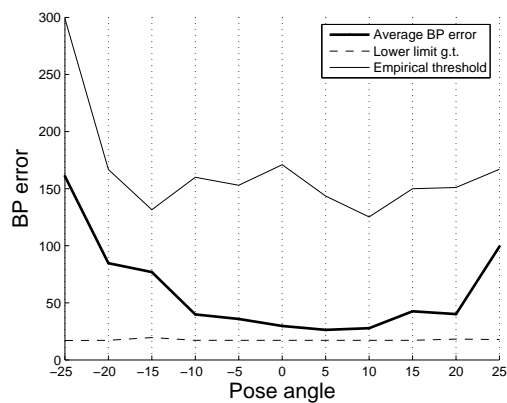
Figure 7.74: Average BP plot (mode of sample) with 20% occlusion.
