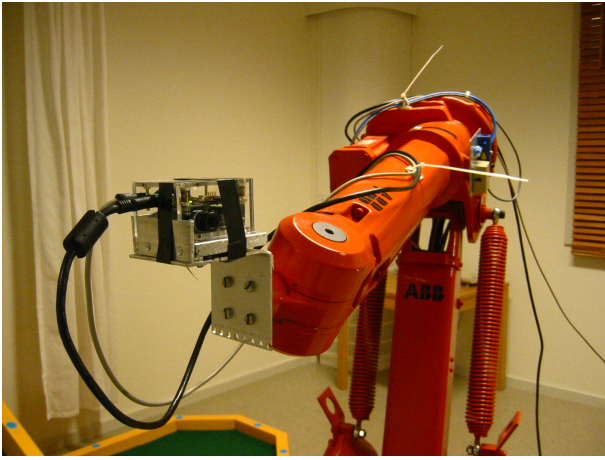
Figure 1. The 6 DoF ABB IRB1400 industrial robot equipped with the custom made sensor.
