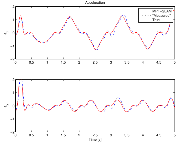
Figure 4. The true acceleration (from the industrial robot), the measured acceleration (from the IMU sensor) and the estimates from Algorithm 1.
